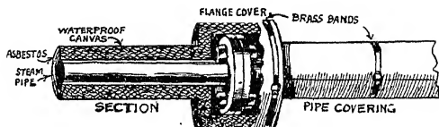
FIG. I.—"VICEROY" COVERING CELLULAR SYSTEM.
